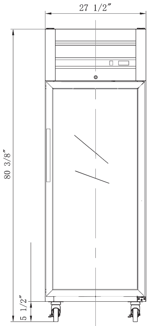
Front View
