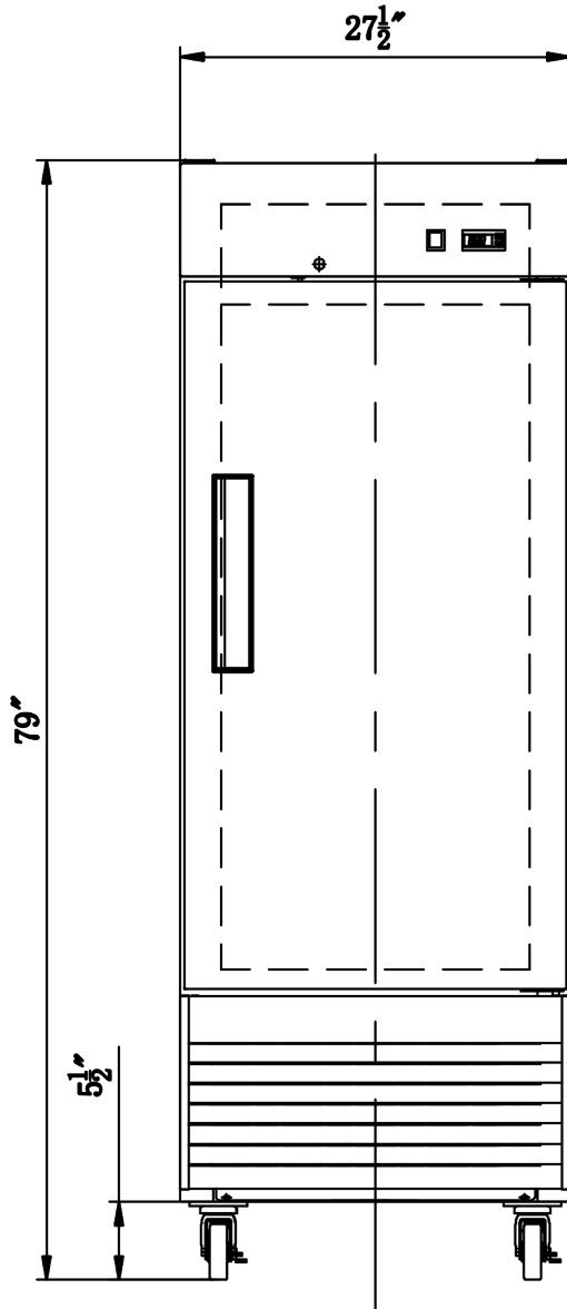
Front View
