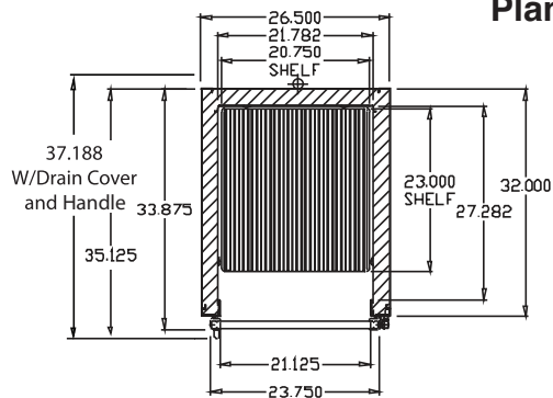
Plan Views
