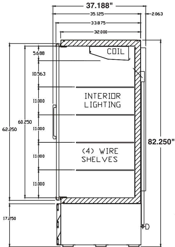
Cross Section
